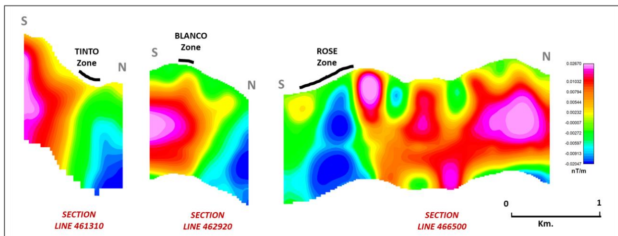
Figure.2: Cross sections through inverted 3D model data on section lines 461310, 462920 and 466500 showing magnetic anomalies underlying known mineralization at the Tinto, Blanco, and Rose zones.
