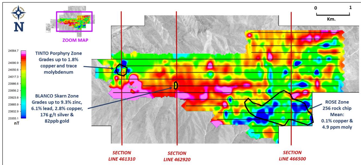
Figure.1: Map of Total Magnetic Intensity (TMI), Reduced to Pole magnetic data. The location of mineralized zones at Rose, Blanco and Tinto are shown relative to the magnetic anomalies. Section Lines 461310, 462920 and 466500 refer to data shown in Figure 2.
