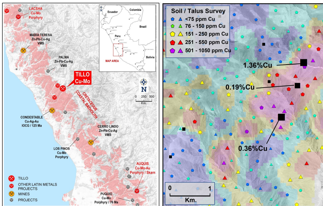
Figure 1: Location of initial rock samples collected at the Tillo copper project.
