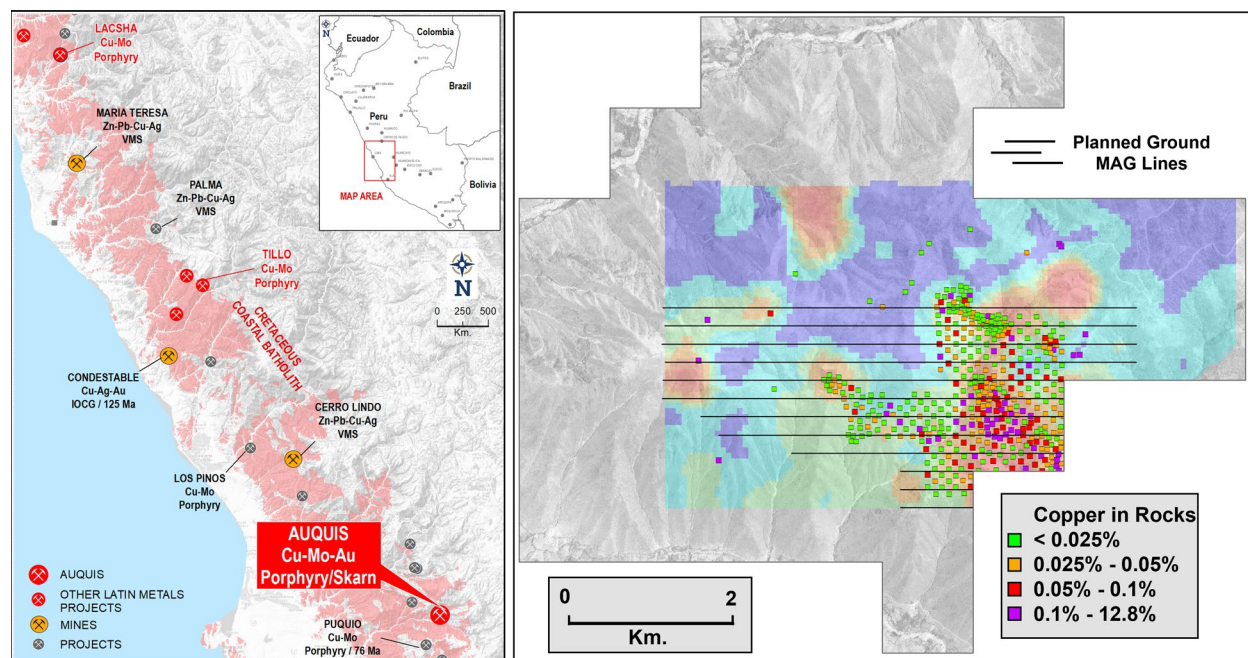
Figure 2: Map of the Auquis copper project showing previously disclosed rock sample analysis and the location of planned ground geophysical survey lines.
