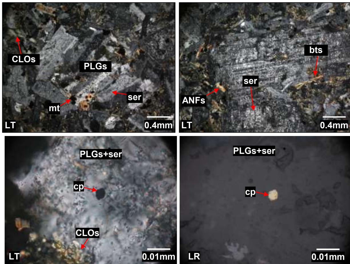
Figure 2: Transmitted light and reflected light; ser (sericite), bts (secondary biotite), mt (magnetite), CLOs (chlorite), cp (chalcopyrite)
