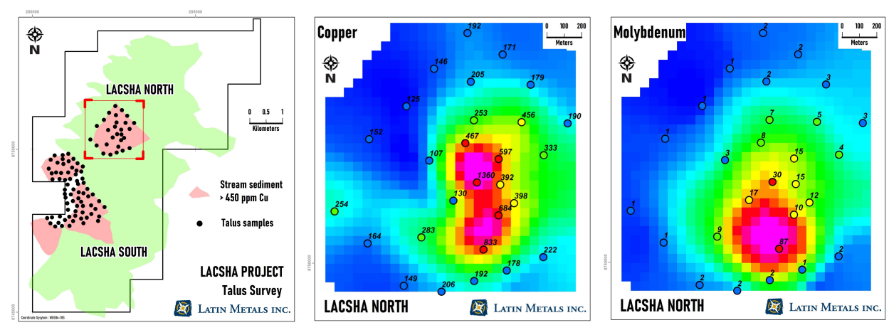
Figure 1: Location of stream sediment anomalies and recent talus samples, and Lacsha North Results for copper and molybdenum.
